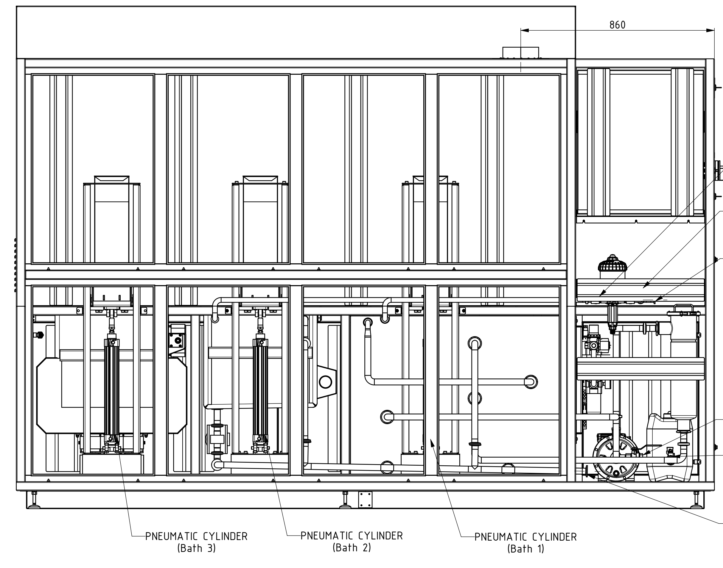
BACK VIEW (without closing plates)
